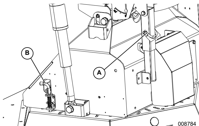
Figure 2-10. Transport Locks
