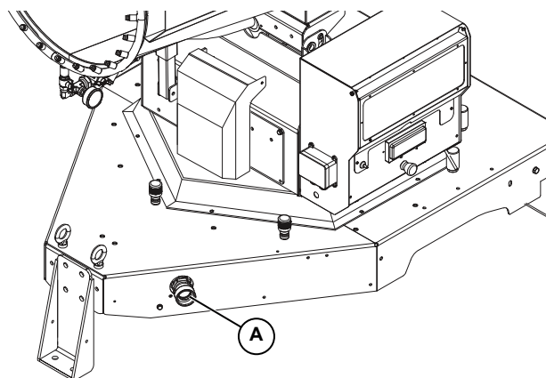
Figure 3-1. Water Connection
