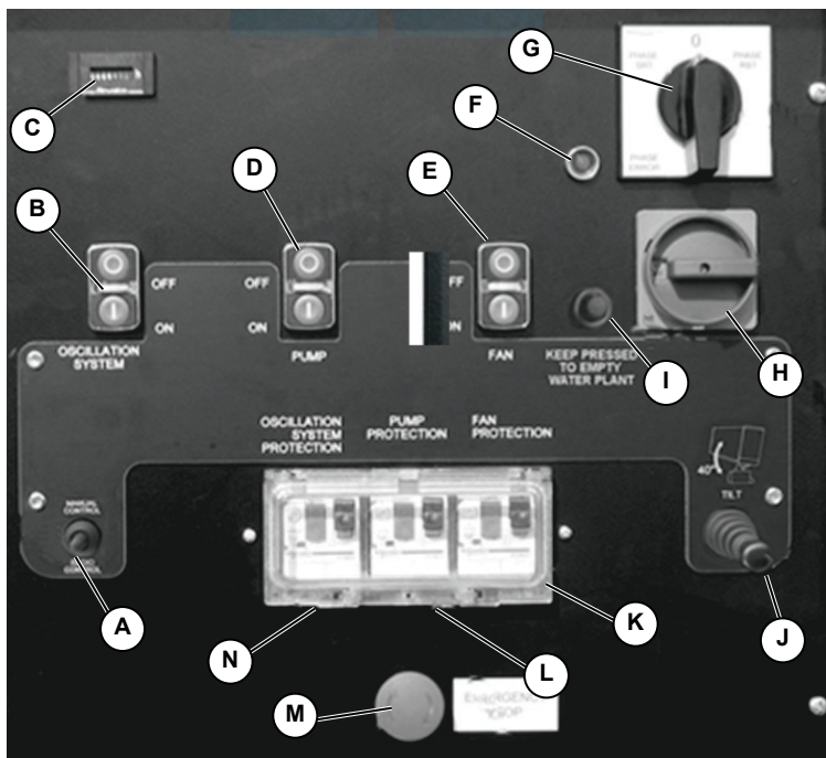
Figure 2-4. Control Panel
