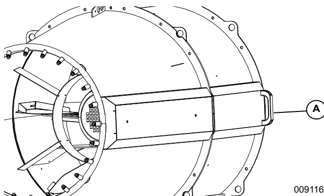
Figure 3-6. Manual rotation
