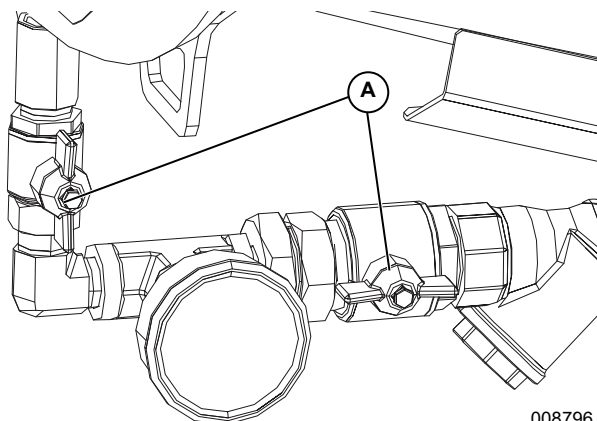
Figure 4-2. Open Valves
