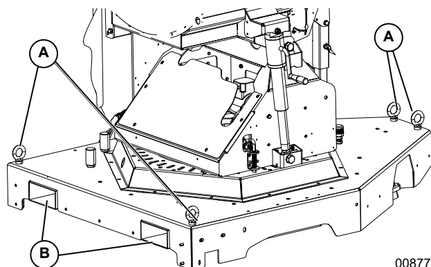
Figure 2-11. Lifting Points
