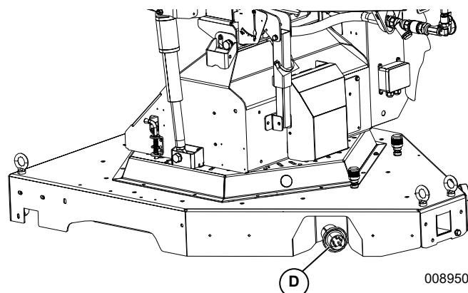
Figure 2-9. Electrical Connection
