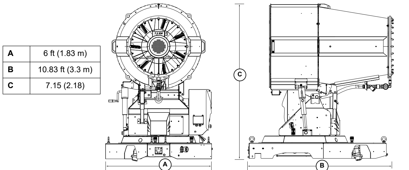
Figure 2-1. Unit Dimensions
